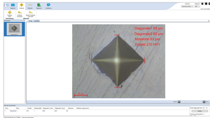
PRESI Touch Essential Automatic or manual measurement of Vickers indents.
